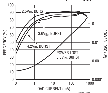
Burst Mode Efficiency, 1.8V OUT
