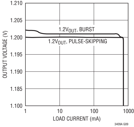
Output Voltage vs Load Current V_{IN} = 1.6\text{V}
