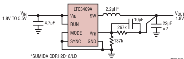
High Efficiency Step-Down Converter
