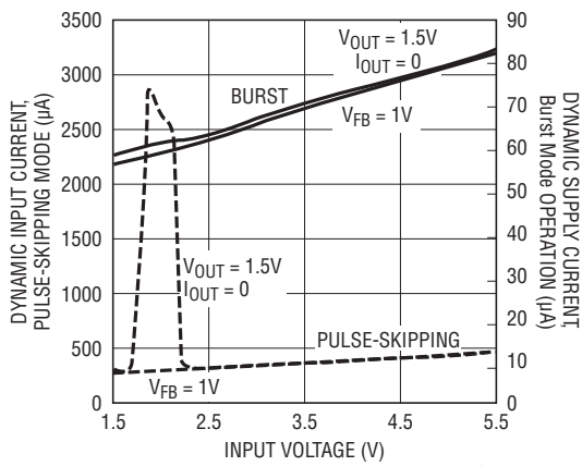
Dynamic Input Current vs Input Voltage
