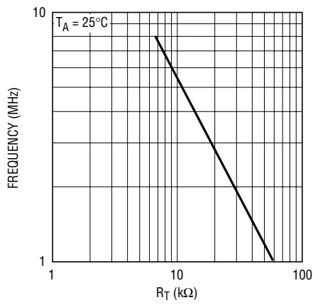
Oscillator Frequency
