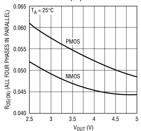
Effective R_{DS(ON)}
