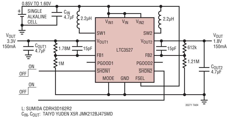
2.2MHz, 1-Cell to V_{OUT1} = 3.3V , V_{OUT2} = 1.8V
