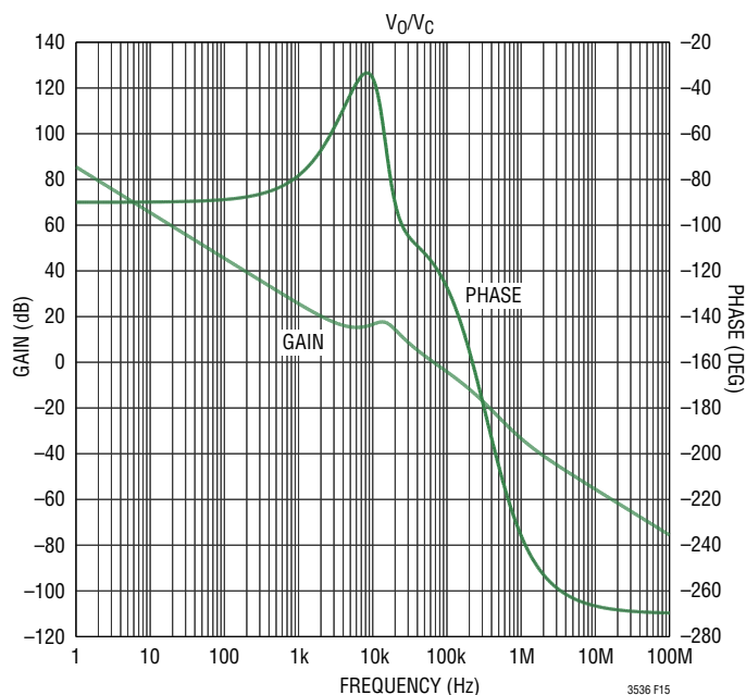
Figure 15. Complete Loop Bode Plot for Buck-Boost Operation Mode
