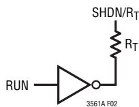
Figure 2. SHDN/RT Pin Activated with a Logic Input
