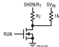
Figure 3. SHDN/RT Pin Activated with a Switch
