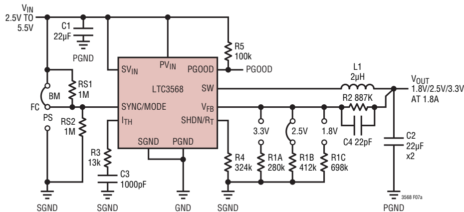
Figure 7. General Purpose Buck Regulator Using Ceramic Capacitors
