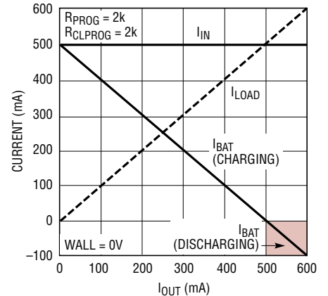
Input and Battery Current vs Output Current
