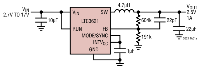
2.5V V_{OUT} with 400mA Burst Clamp, f_{sw} = 1\text{MHz}
