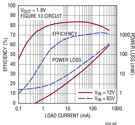
Efficiency and Power Loss vs Load Current, V OUT = 1.8V
