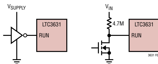
Figure 7. RUN Pin Interface to Logic
