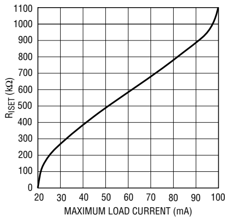
Figure 1. R_{ISET} Selection
