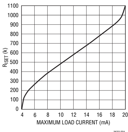
Figure 1. R_{ISET} Selection
