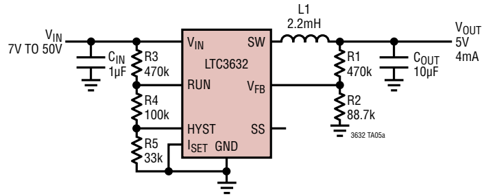
Small Size, Limited Peak Current, 4mA Regulator
