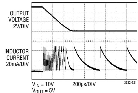
Short-Circuit Response
