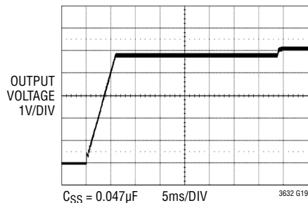
Soft-Start Waveforms
