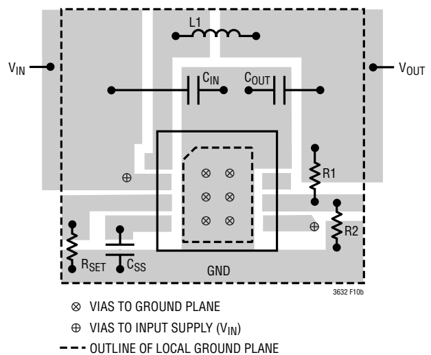
Figure 10. Layout Example
