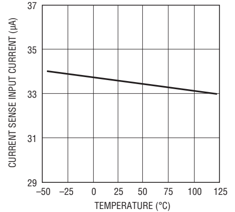
Current Sense Pin Input Current vs Temperature
