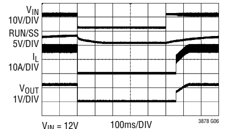
Start-Up V_{IN} Cycled Low and High
