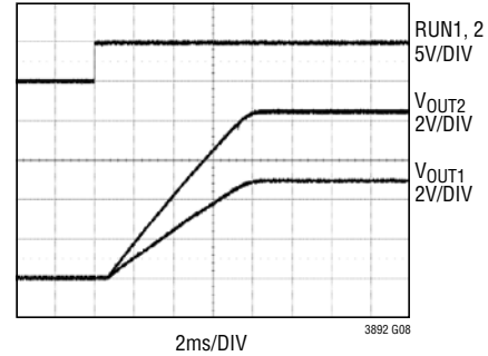
FIGURE 13 CIRCUIT
