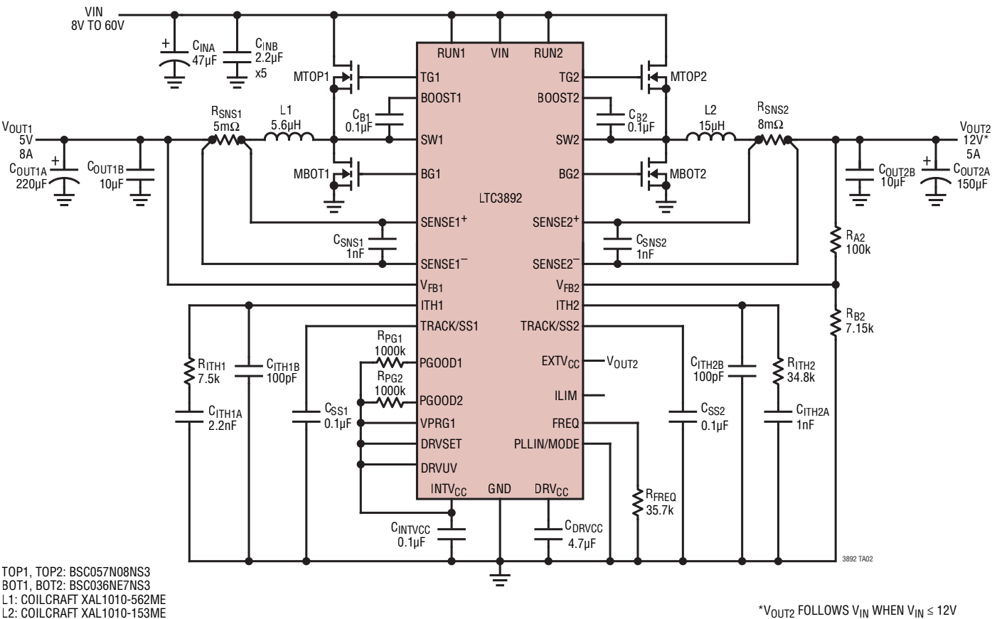
Figure 11. High Efficiency Dual 5V/12V Step-Down Converter with 10V Gate Drive
