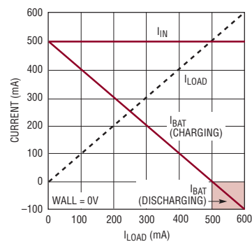
Input and Battery Current vs Load Current
