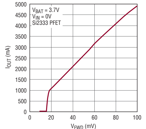
Ideal Diode Resistance and Current vs Forward Voltage with External Device
