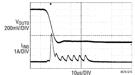
FIGURE 44 CIRCUIT AT 12\text{V}_{\text{IN}} , NO LOAD ON \text{V}_{\text{OUT}0} PRIOR TO APPLICATION OF SHORT CIRCUIT
