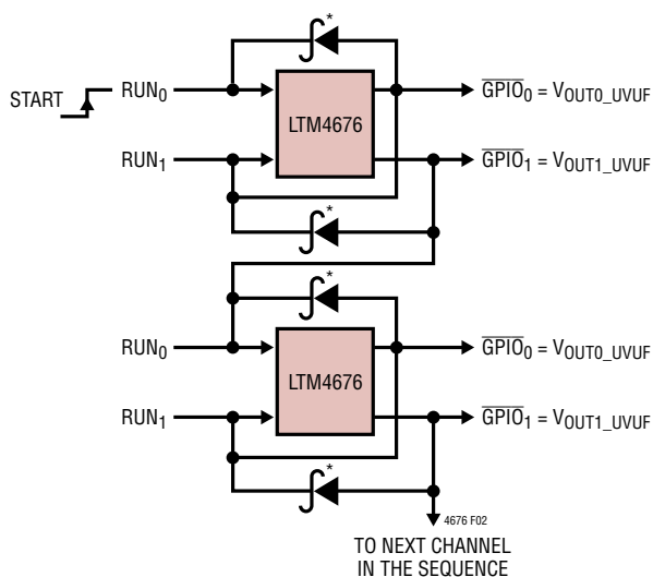
Voltage Based Sequencing by Cascading \overline{\text{GPIO}}_n Pins Into \text{RUN}_n Pins ( \text{MFR\_GPIO\_PROPAGATE} = \text{XXX1X00X00XXXX}_b and \text{MFR\_GPIO\_RESPONSE} = 0x00 )
