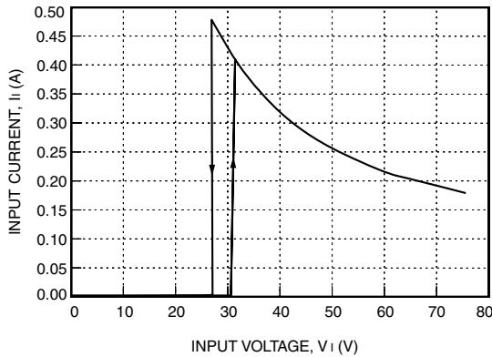
Figure 3. LW010 Input Current vs. Input Voltage at I_o = I_{o, max} and T_c = 25^\circ C
