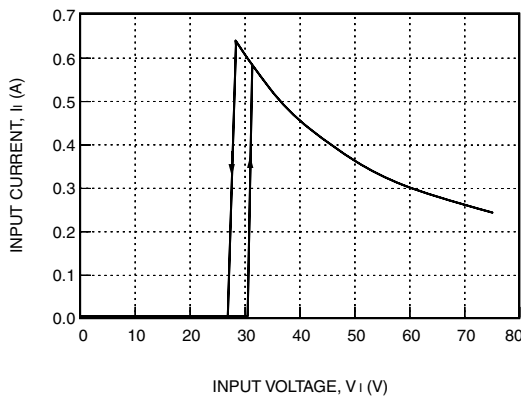
Figure 4. LW015 Input Current vs. Input Voltage at I_o = I_{o, max} and T_c = 25^\circ C
