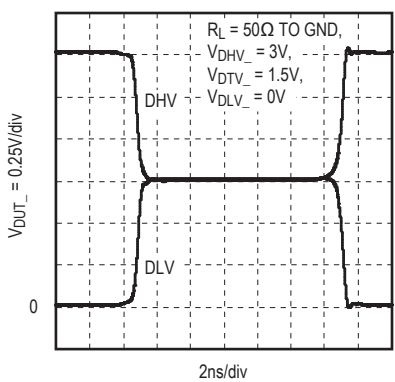
DRIVER-TO-TERM TRANSITION
