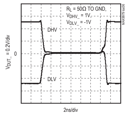
DRIVER TO HIGH-IMPEDANCE TRANSITION
