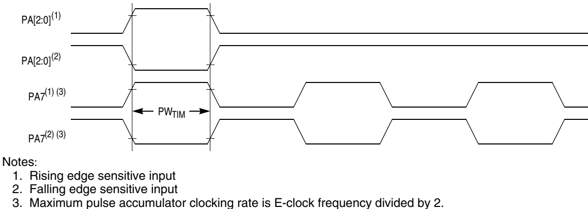
Figure 10-2. Timer Inputs
