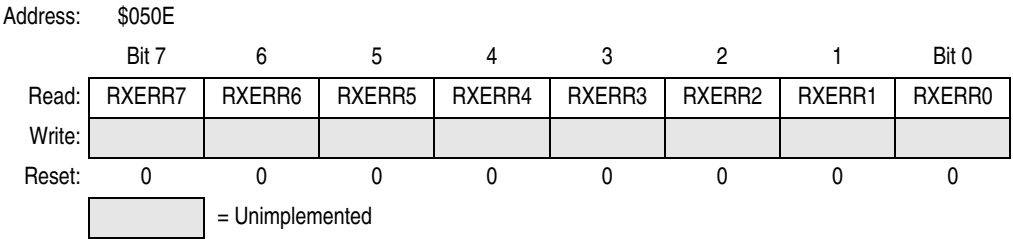
Figure 12-25. Receiver Error Counter (CRXERR)
