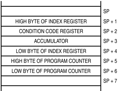
Figure 20-15. Stack Pointer at Monitor Mode Entry
