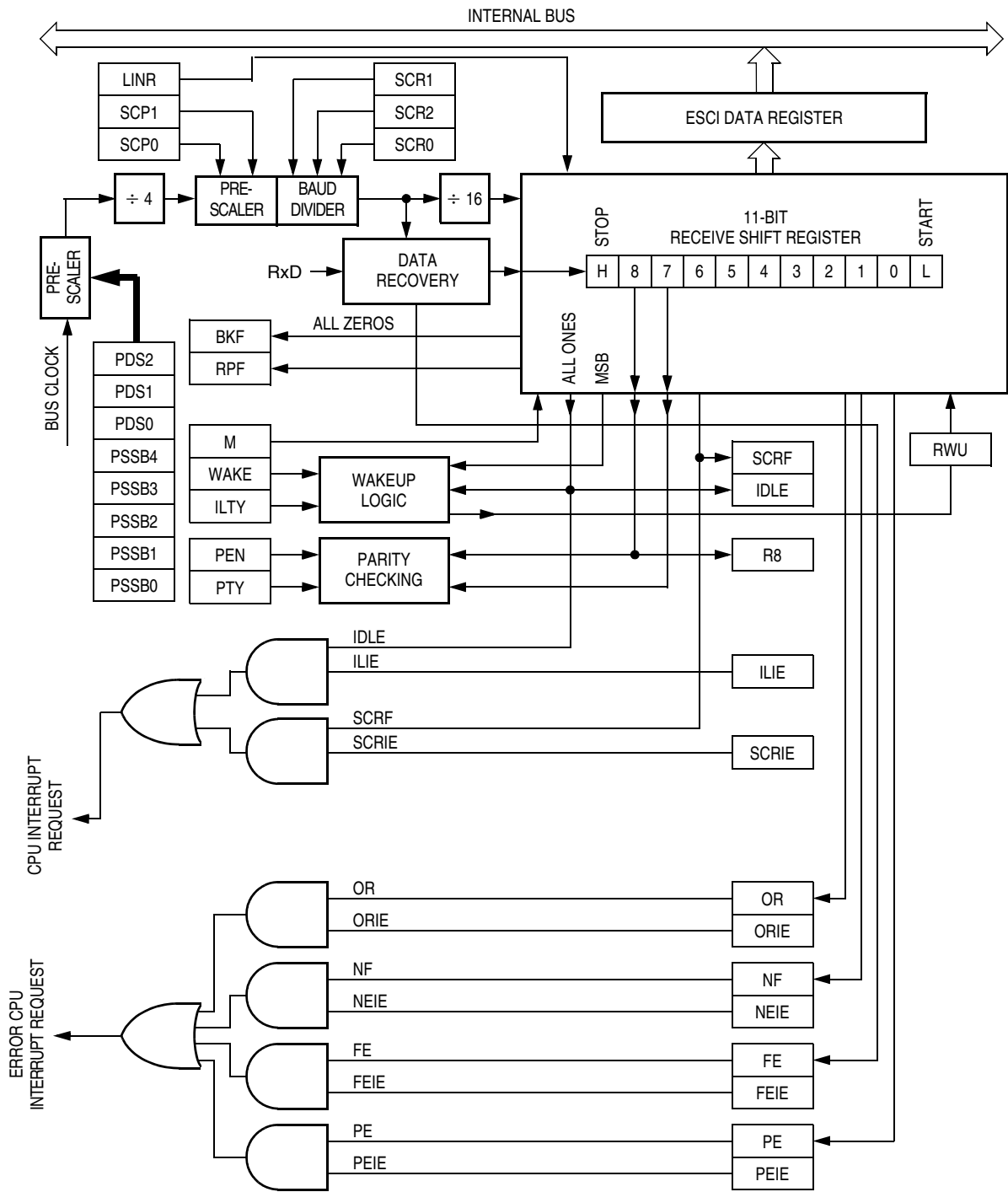
Figure 15-6. ESCI Receiver Block Diagram
