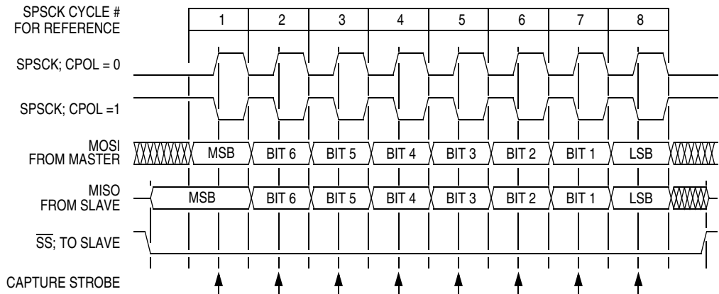
Figure 17-5. Transmission Format (CPHA = 0)
