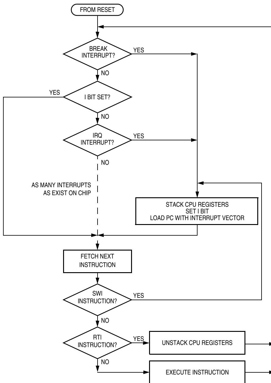
Figure 16-10. Interrupt Processing
