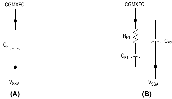
Figure 4-9. PLL Filter
