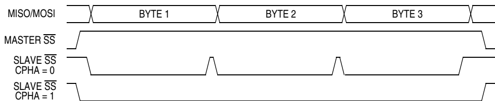
Figure 17-6. CPHA/ \overline{SS} Timing
