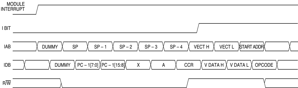
Figure 16-8. Interrupt Entry Timing
