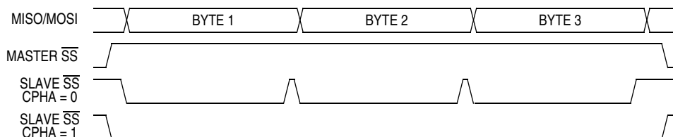
Figure 17-13. CPHA/ \overline{SS} Timing
