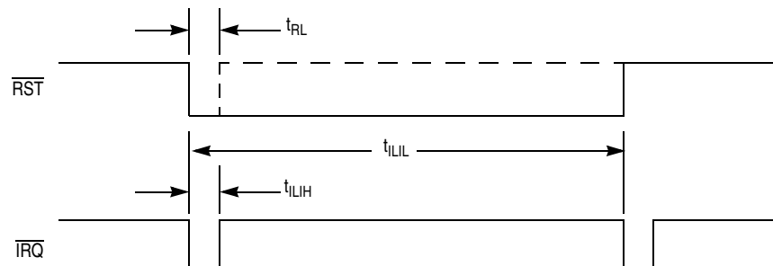
Figure 21-1. \overline{RST} and \overline{IRQ} Timing
