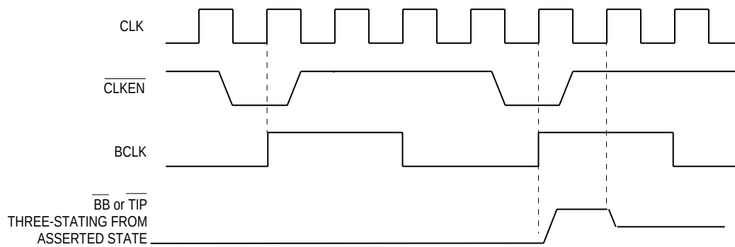
Figure 7-4. Quarter-Speed Clock
