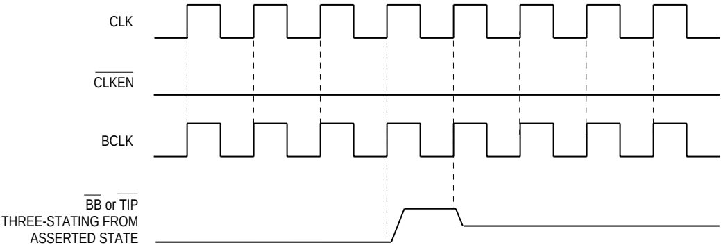
Figure 7-2. Full-Speed Clock
