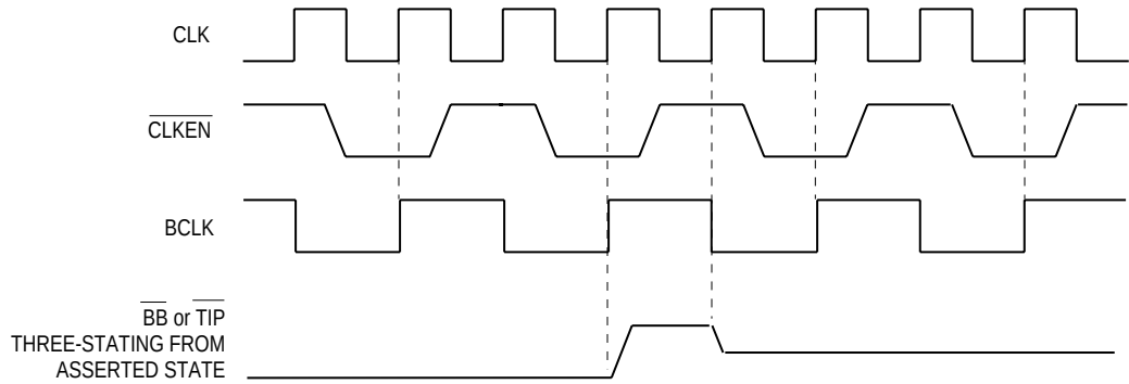
Figure 7-3. Half-Speed Clock
