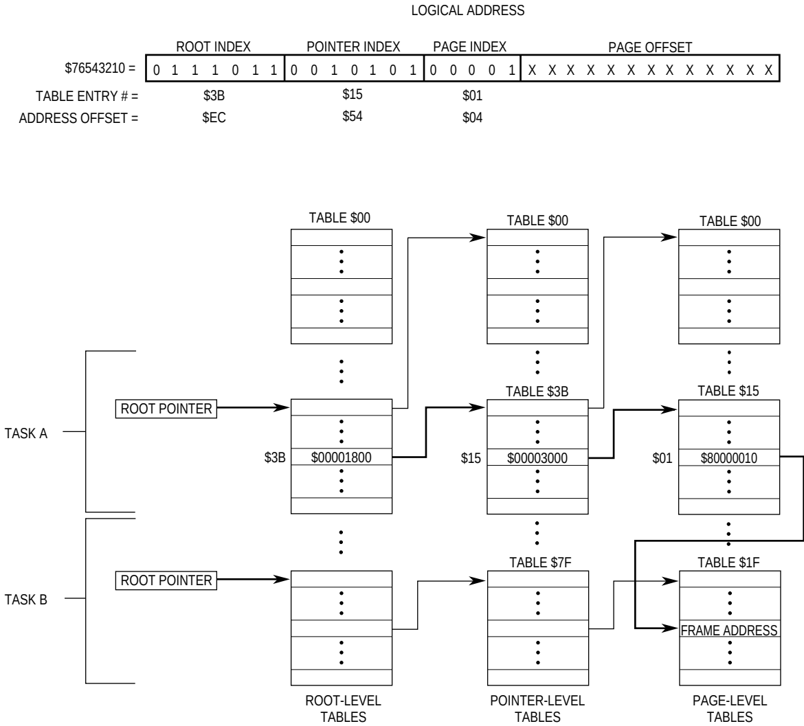
Figure 4-13. Translation Table Using Indirect Descriptors
