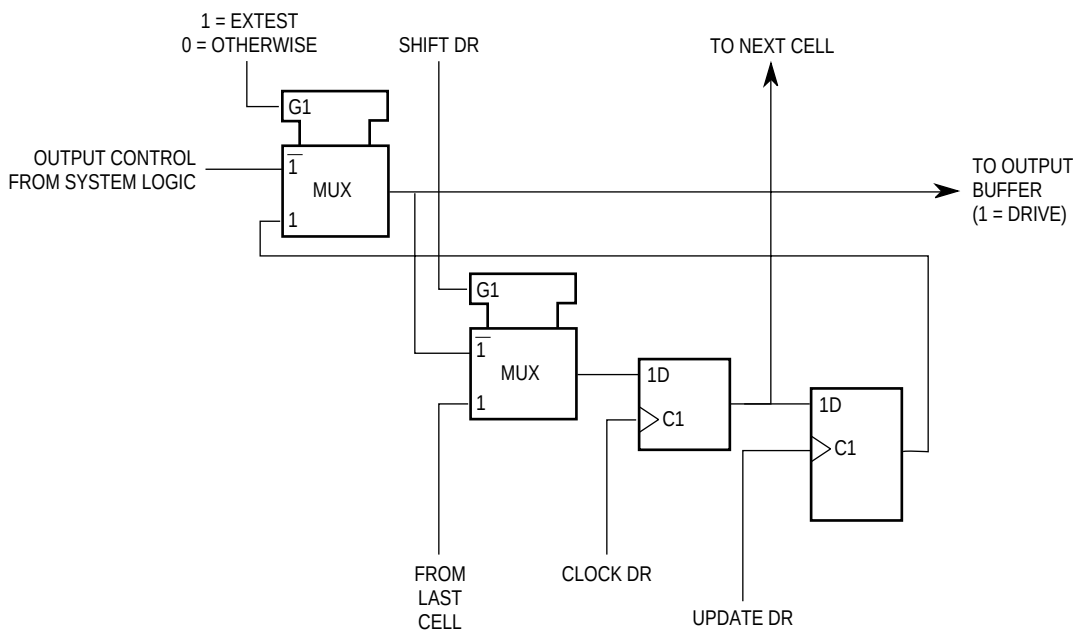
Figure 9-6. Output Control Cell (IO.Ctl)
