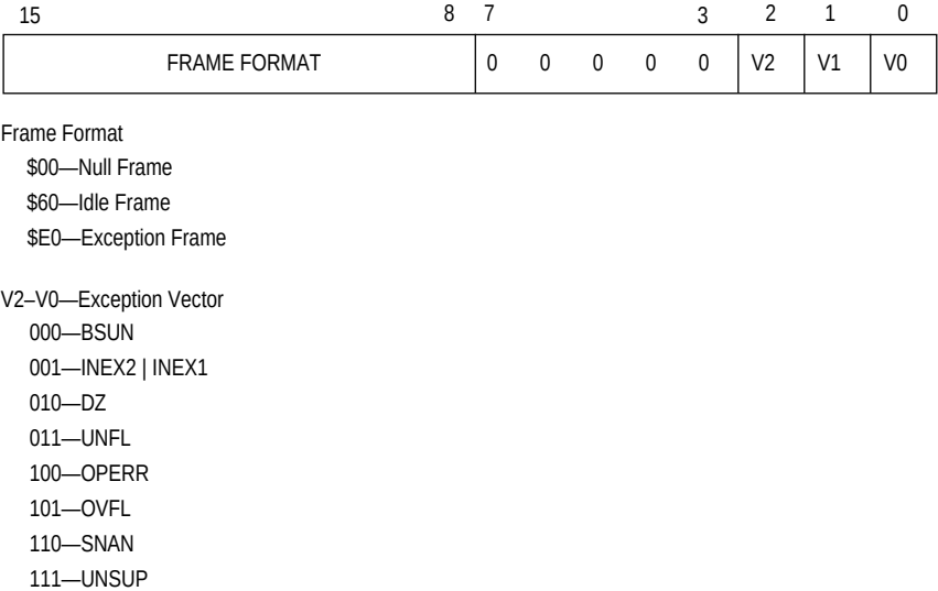
Figure 6-11. Status Word Contents
