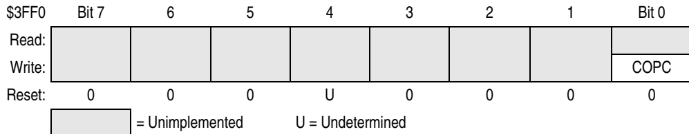
Figure 5-6. COP Clear Register (COPCLR)
