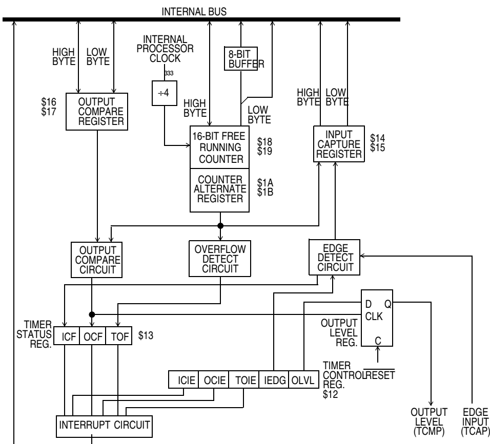
Figure 8-1. Capture/Compare Timer Block Diagram
