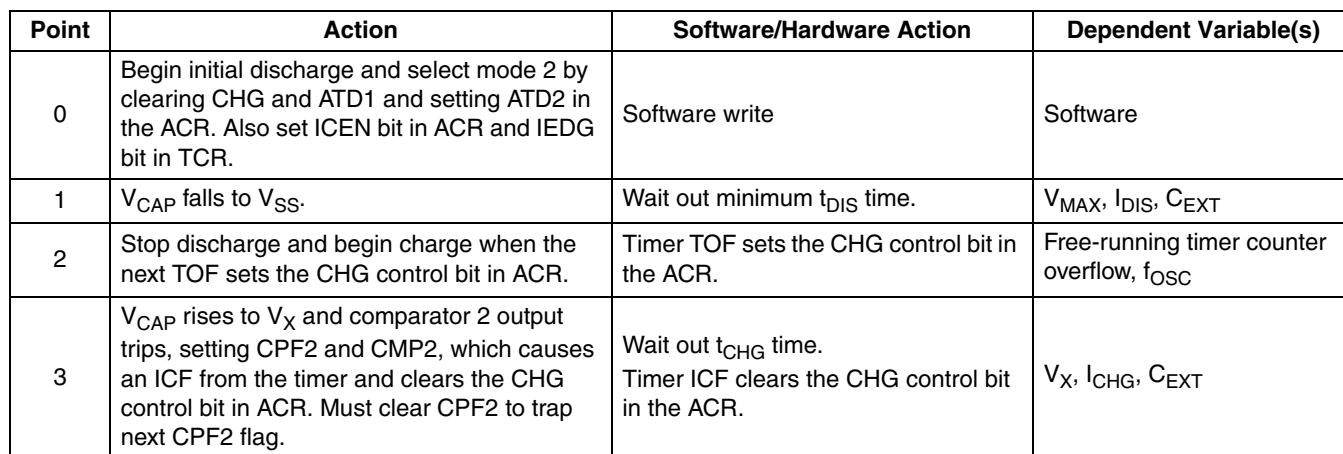
Figure 8-10. A/D Conversion — TOF/ICF Control (Mode 2)
