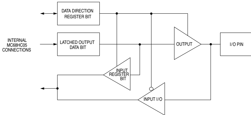
Figure 3-1 Port I/O Circuitry
