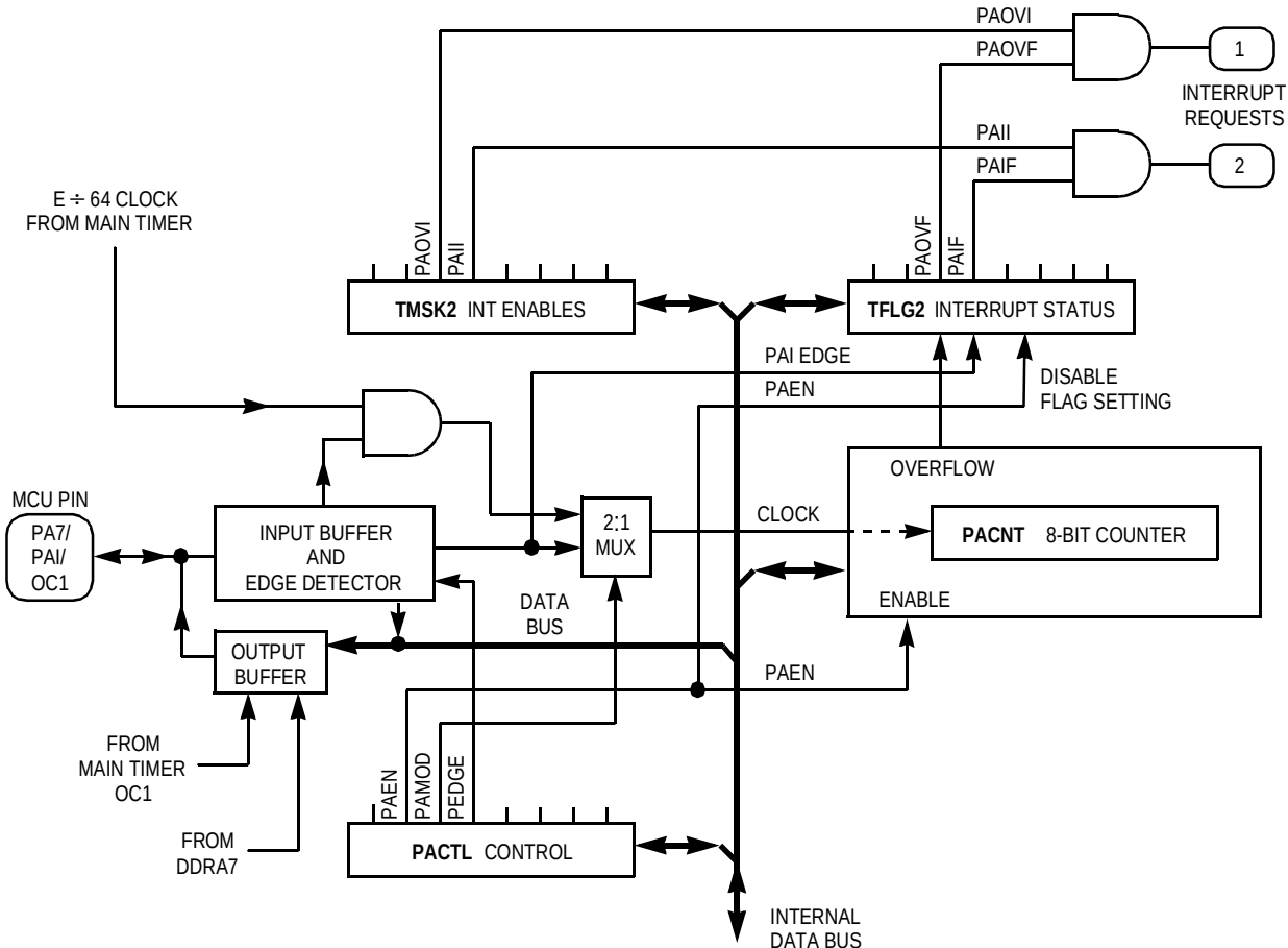
Figure 9-24. Pulse Accumulator
