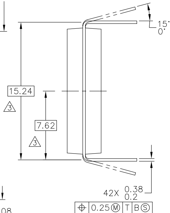
END VIEW
