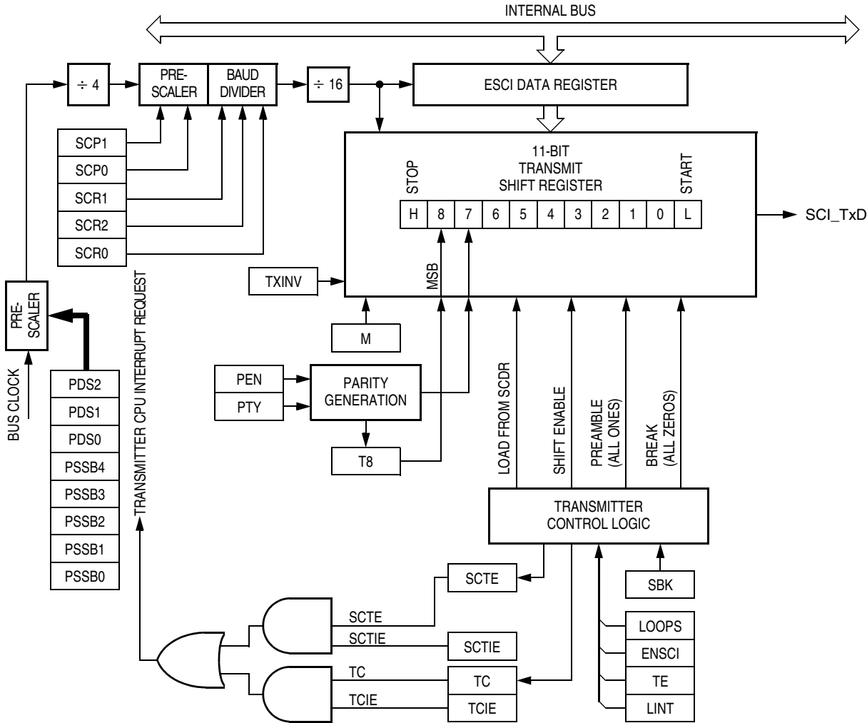
Figure 15-5. ESCI Transmitter
