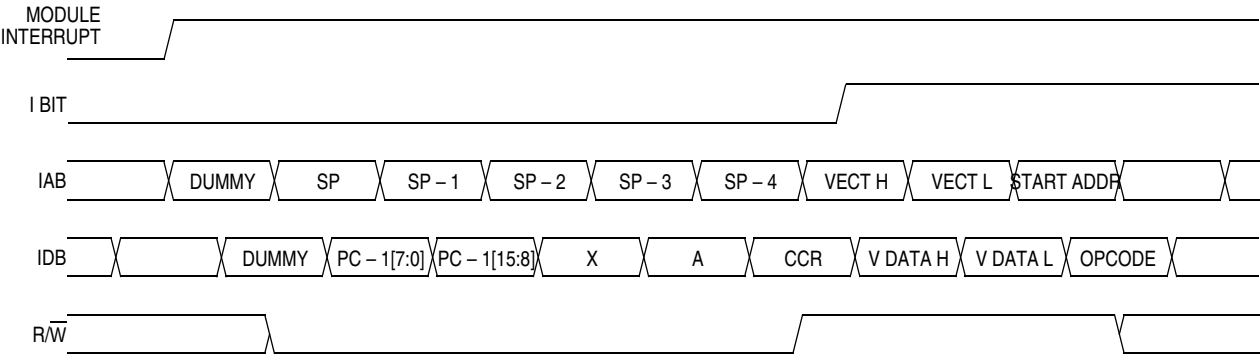
Figure 13-7. Interrupt Entry
