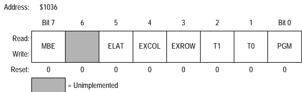
Figure 4-15. MC68HC711E20 EPROM Programming Control Register (EPROG)
