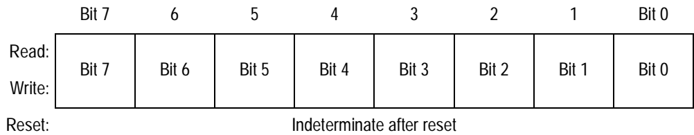
Figure 9-5. Timer Input Capture 2 Register Pair (TIC2)
