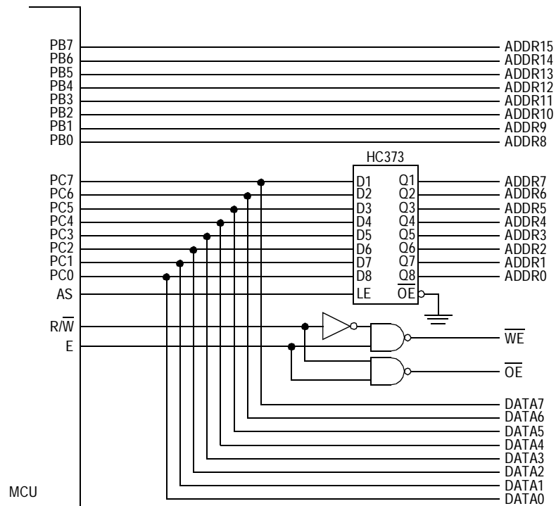
Figure 4-1. Address/Data Demultiplexing
