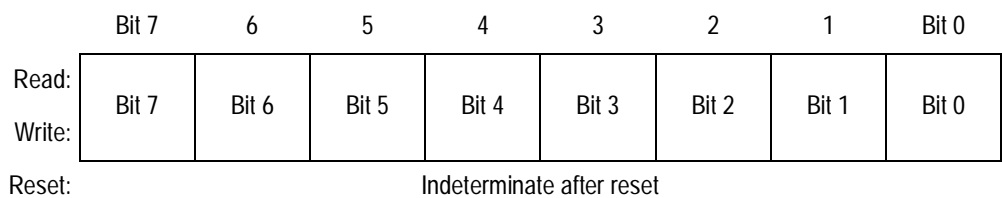
Figure 9-6. Timer Input Capture 3 Register Pair (TIC3)
