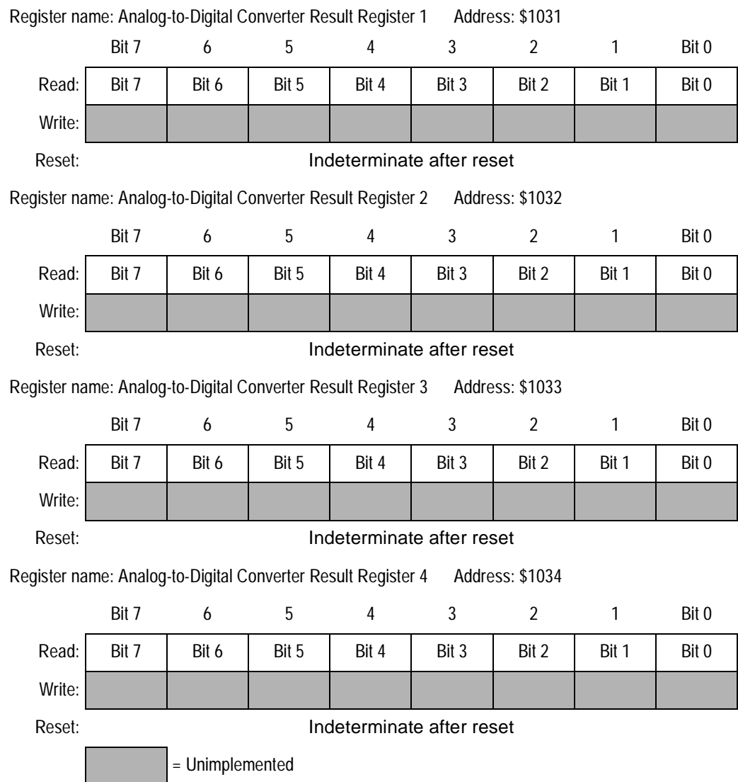
Figure 10-6. Analog-to-Digital Converter Result Registers (ADR1–ADR4)
