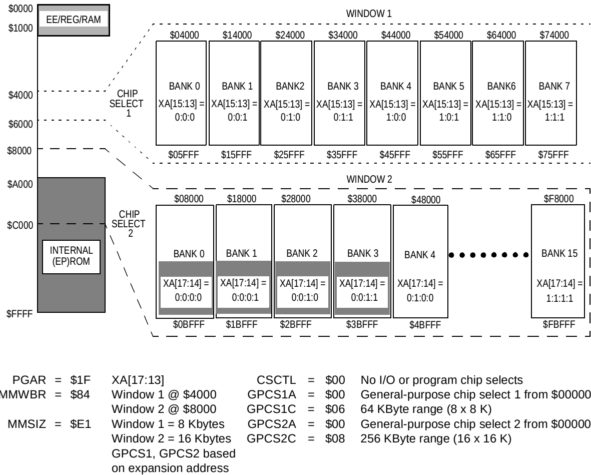
Figure 11-16. Memory Expansion Example 2 (Sheet 1 of 2) Memory Map for One 8-Kbyte Window with Eight Banks and One 16-Kbyte Window with 16 Banks of External Memory
