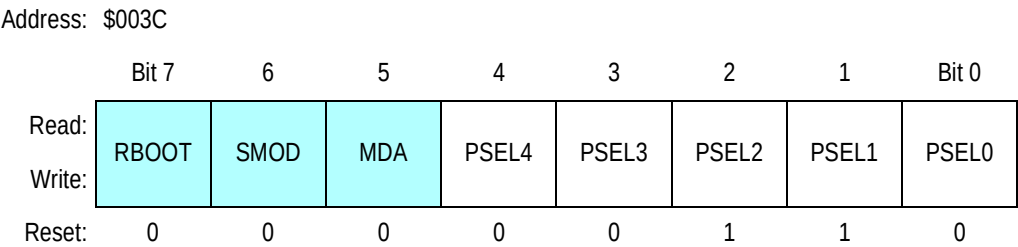
Figure 5-7. Highest Priority I-Bit Interrupt and Miscellaneous Register (HPRIO)
