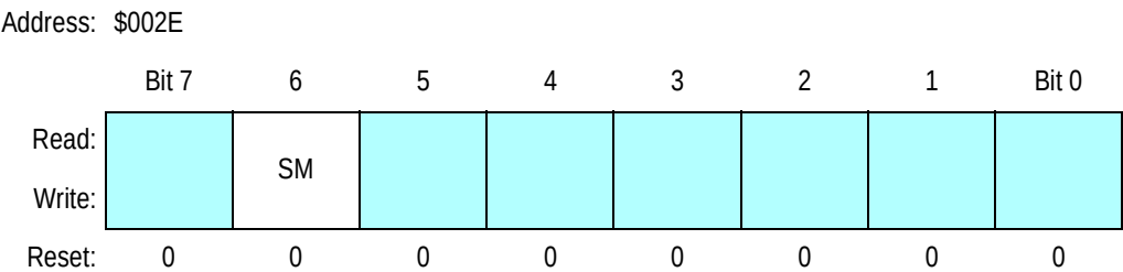
Figure 5-12. System Configuration Options 3 Register (OPT3)
