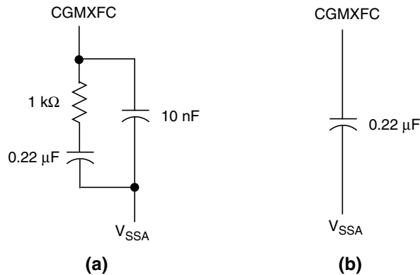
Figure 6-10. PLL Filter
