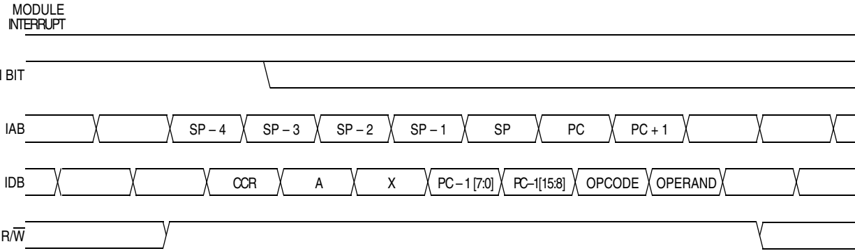
Figure 7-9. Interrupt Recovery
