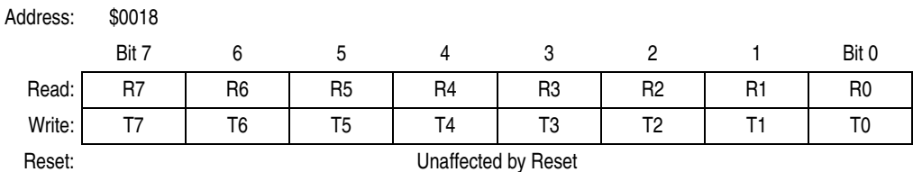
Figure 16-17. SCI Data Register (SCDR)
