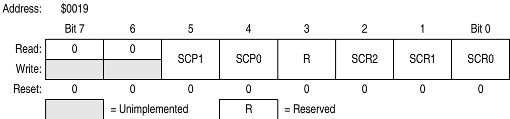
Figure 16-18. SCI Baud Rate Register (SCBR)
