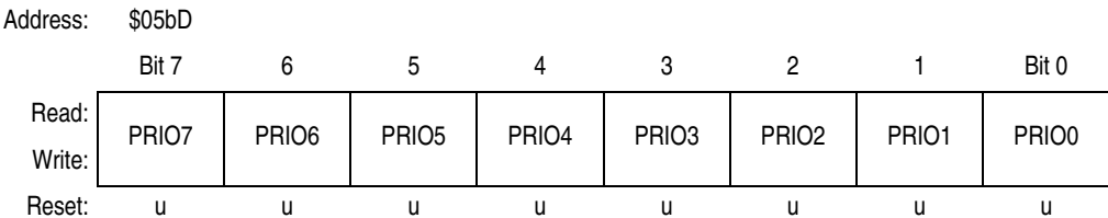
Figure 24-13. Transmit Buffer Priority Register (TBPR)
