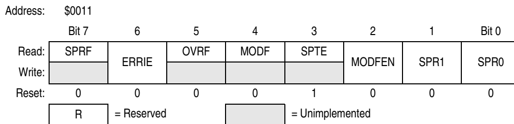
Figure 17-13. SPI Status and Control Register (SPSCR)
