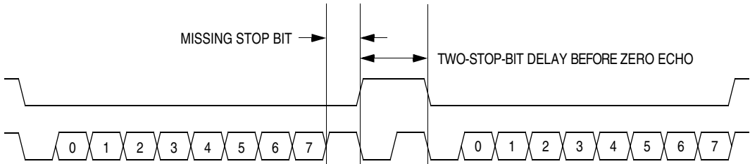
Figure 12-5. Break Transaction
