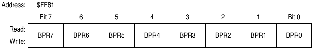
Figure 5-2. FLASH-2 Block Protect Register (FL2BPR)
