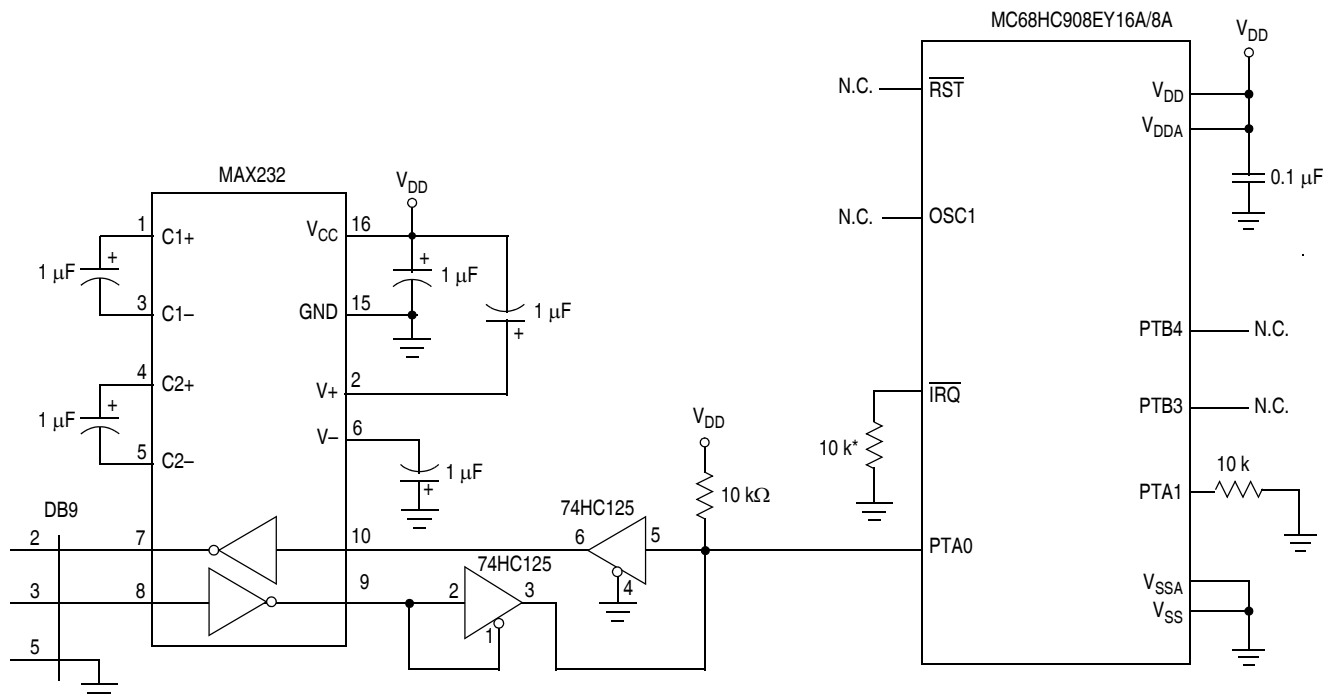
Figure 19-11. Forced Monitor Mode ( V_{\overline{\text{IRQ}}} = V_{\text{SS}} )
