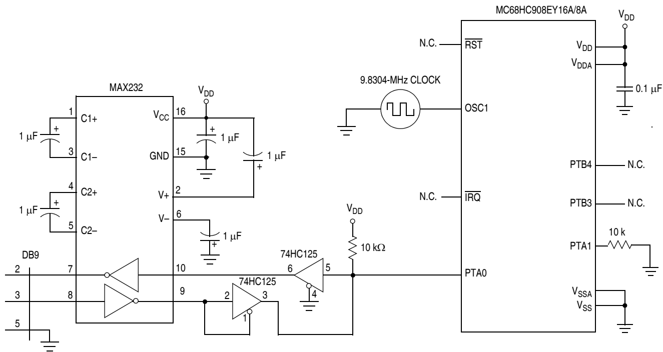
Figure 19-10. Forced Monitor Mode ( V_{IREQ} = V_{DD} )
