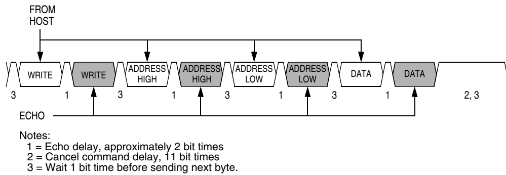
Figure 16-16. Write Transaction
