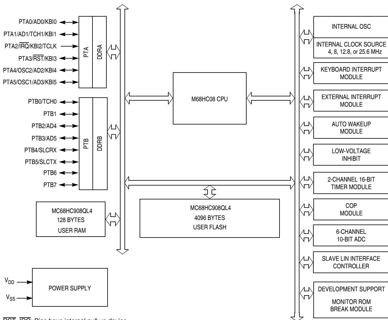
Figure 1-1. Block Diagram
