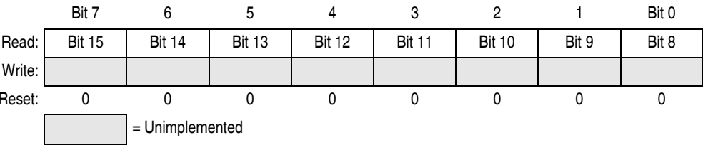
Figure 15-5. TIM Counter High Register (TCNTH)
