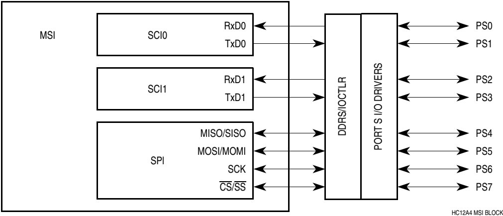
Figure 16-1. Multiple Serial Interface Block Diagram
