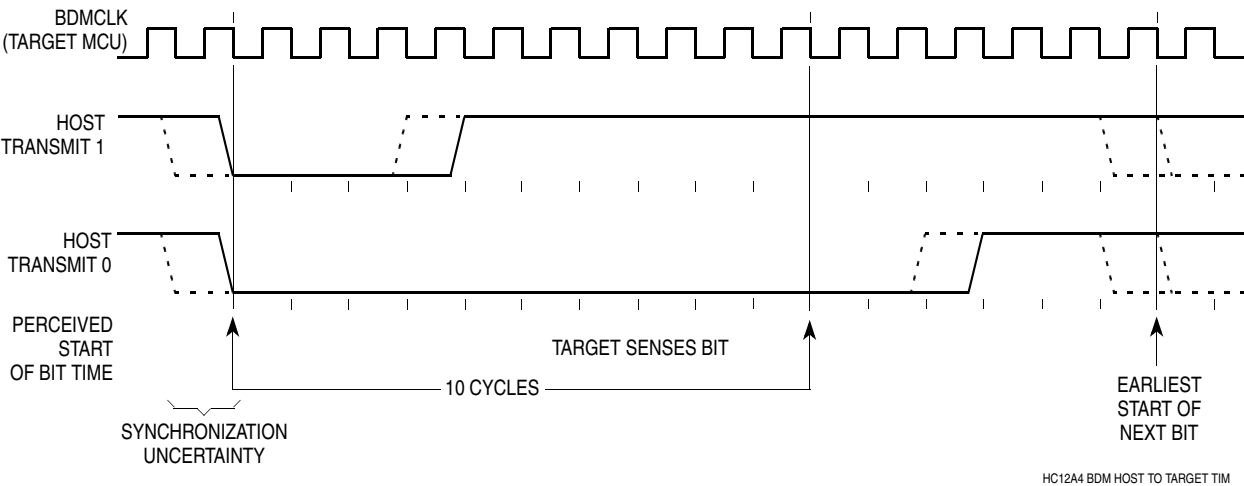
Figure 20-1. BDM Host to Target Serial Bit Timing
