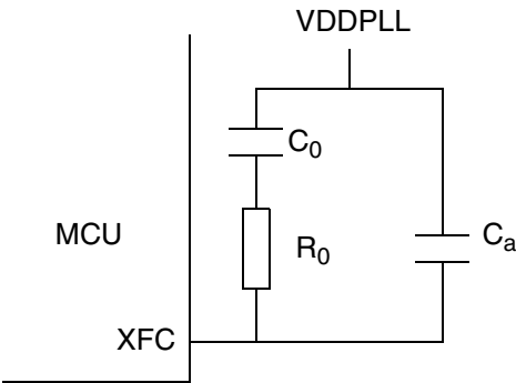
Figure 3-4. PLL Loop Filter Connections
