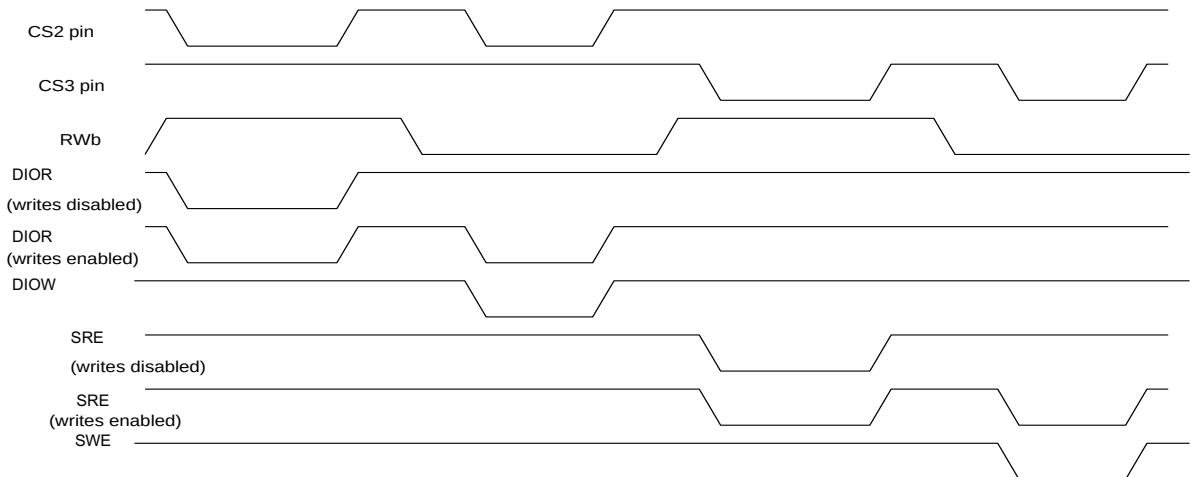
Figure 13-3 DIOR and SRE Timing Diagram
