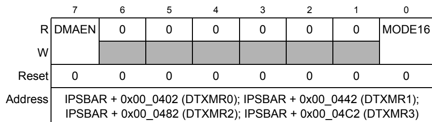
Figure 22-3. DMA Timer Extended Mode Registers (DTXMR n )
