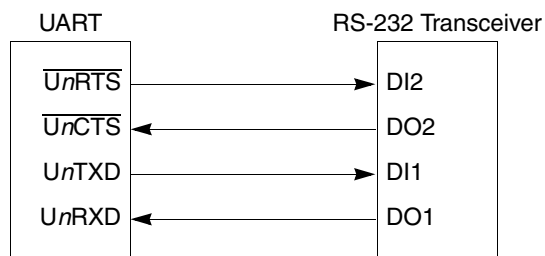
Figure 24-2. UART/RS-232 Interface
