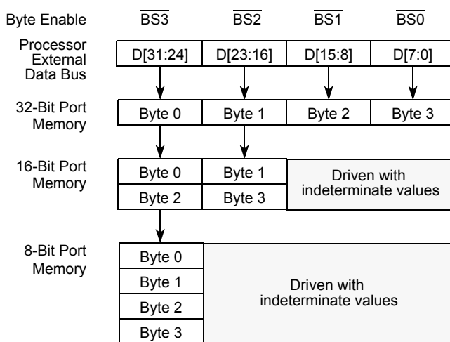
Figure 18-5. SDRAM connections for port sizes of 32, 16, or 8 bits
