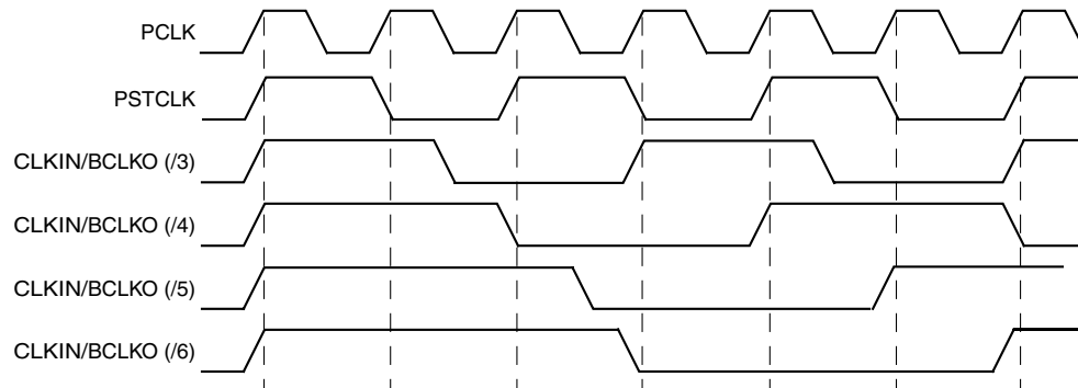
Figure 7-3. CLKIN, PCLK, PSTCLK, and BCLKO Timing
