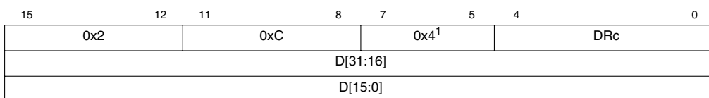
Figure 5-44. WDMREG BDM Command Format
