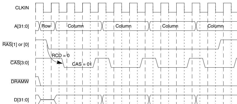
Figure 11-8. Burst Page-Mode Write Operation (4-3-3-3)
