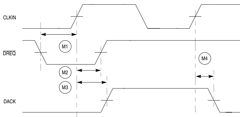
Figure 20-23. DMA Timing
