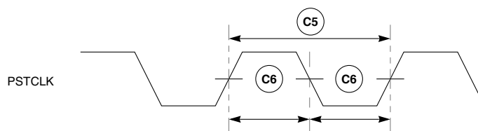
Figure 20-5. PSTCLK Timing
