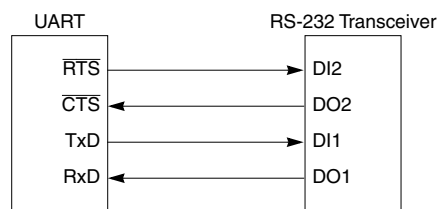
Figure 14-25. UART/RS-232 Interface
