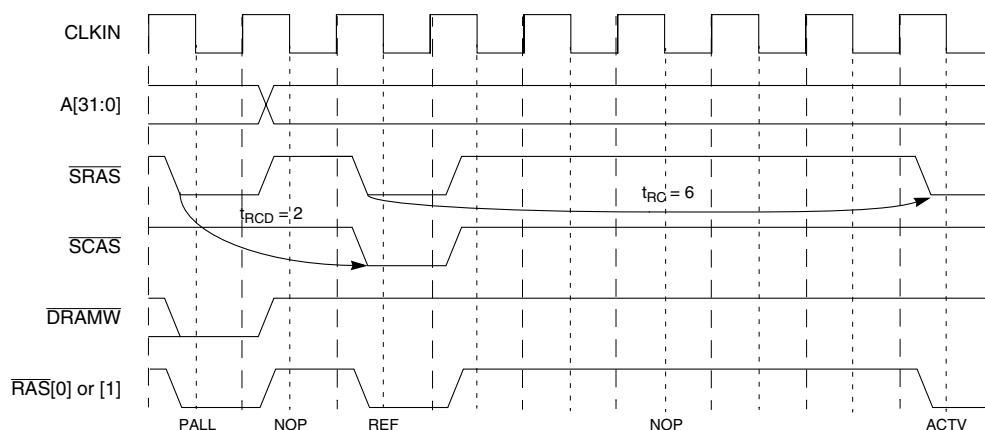
Figure 11-22. Auto-Refresh Operation
