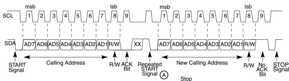
Figure 8-3. Repeated START
