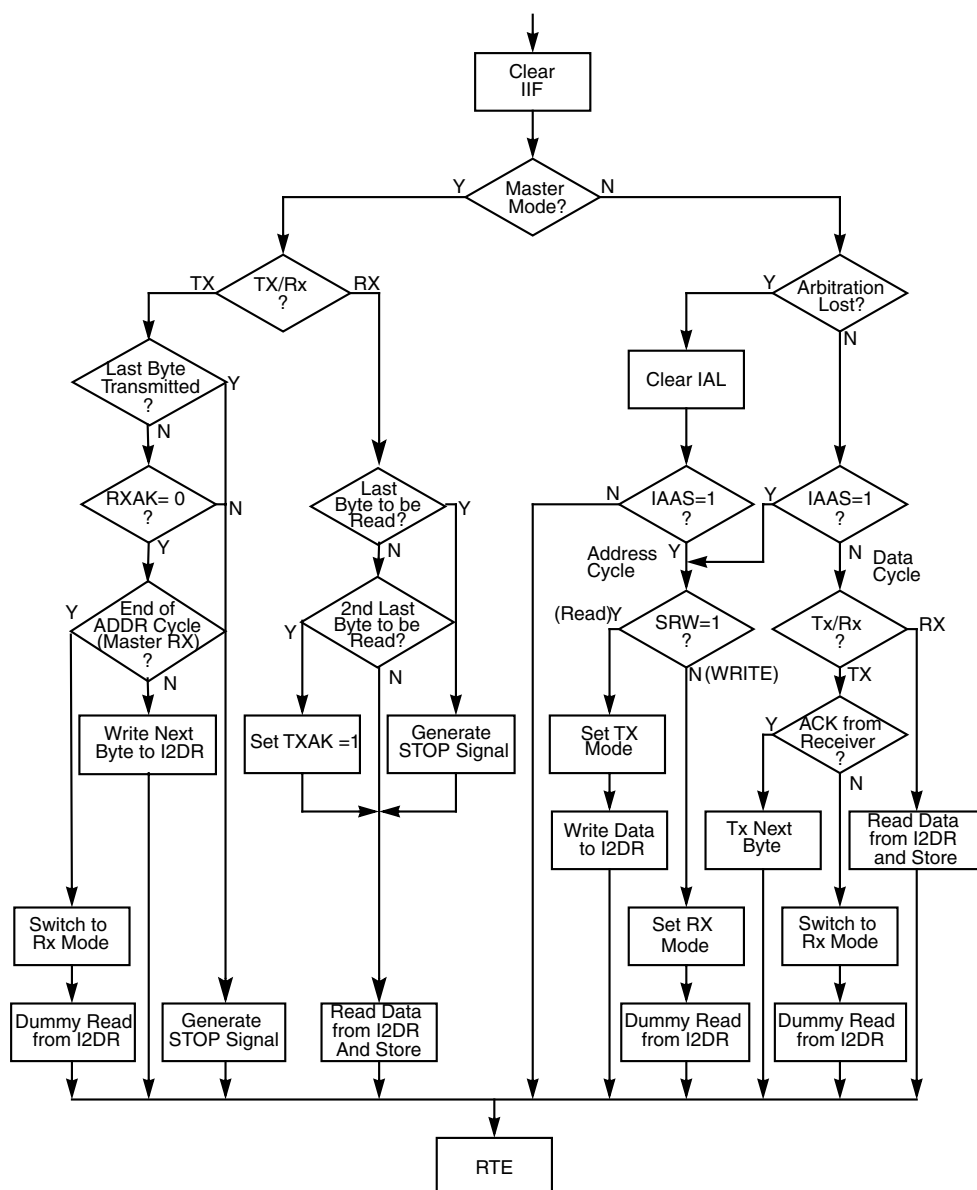
Figure 8-10. Flow-Chart of Typical I²C Interrupt Routine
