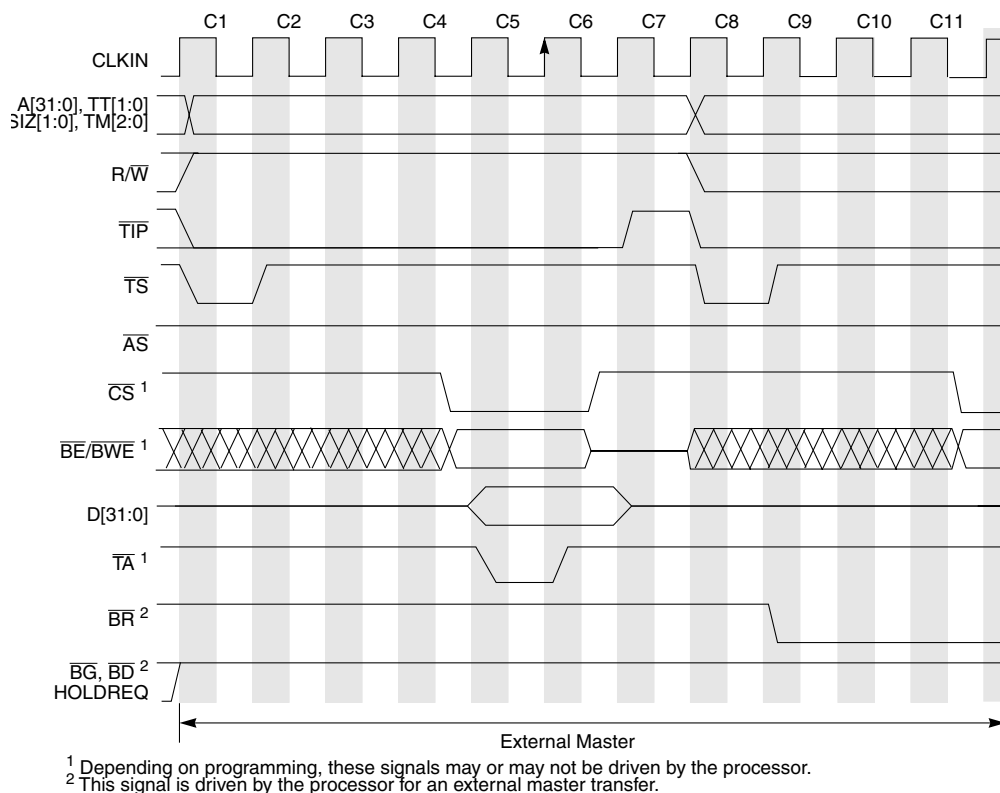
Figure 18-24. Basic No-Wait-State External Master Access
