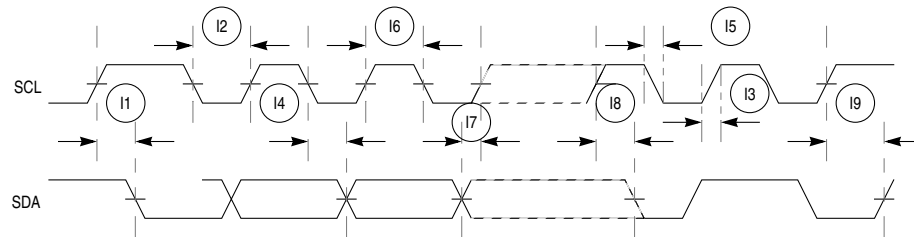
Figure 20-18. I²C Input/Output Timings
