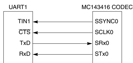
Figure 14-26. UART1/CODEC Interface
