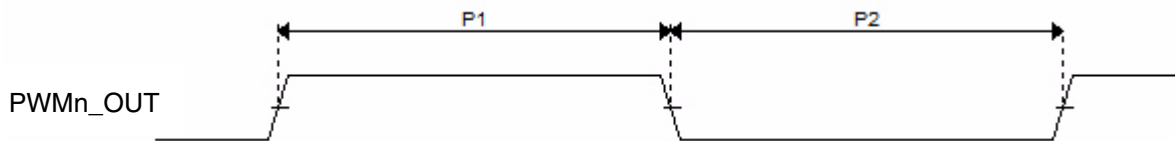
Figure 89. PWM Timing
