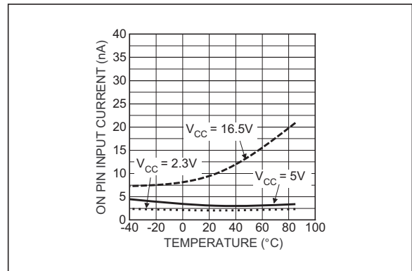
FIGURE 2-18: ON Input Current vs. Temperature.
