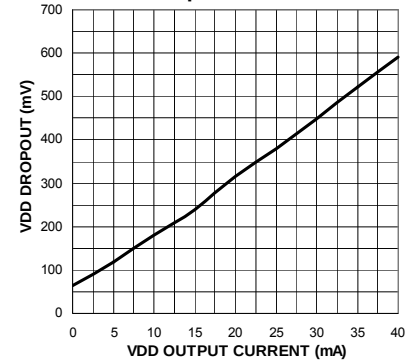
VDD Dropout vs. VDD Load
