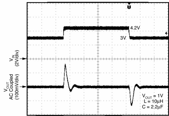
Line Transient
