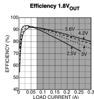
Figure 2. Efficiency Curve
