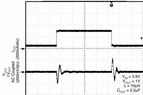
Load Transient
