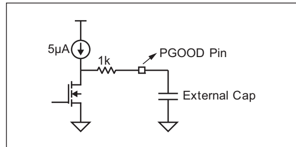
FIGURE 4-1: Power Good Circuit.
