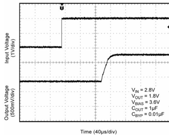
Turn-on Time
