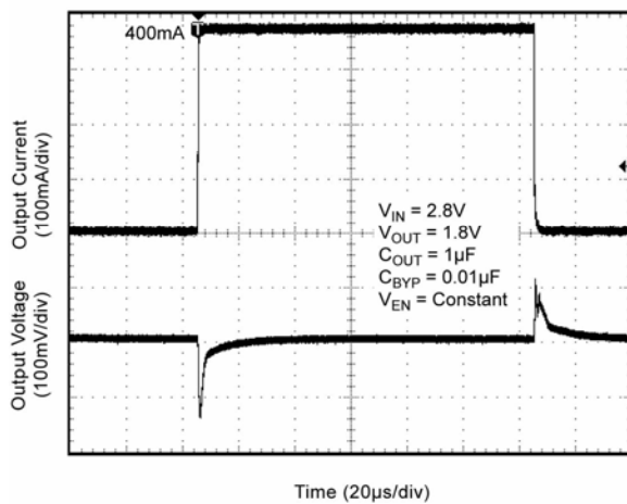
Load Transient ( V_{IN} )
