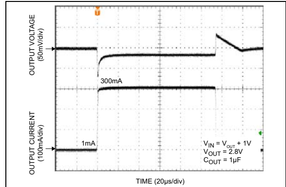
FIGURE 2-11: Load Transient.
